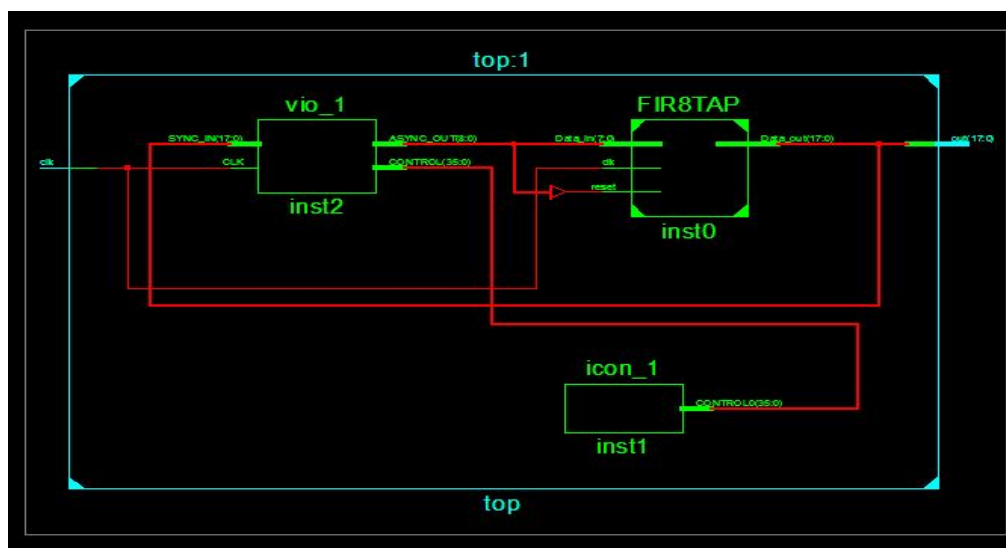
Figure 7: RTL Schematic view of 8 tap FIR filter
