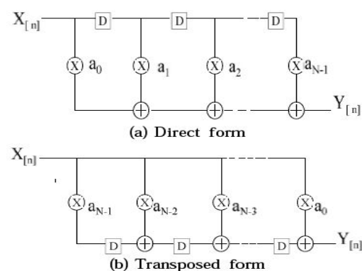
Figure 2: Various Realizations of FIR Filters
