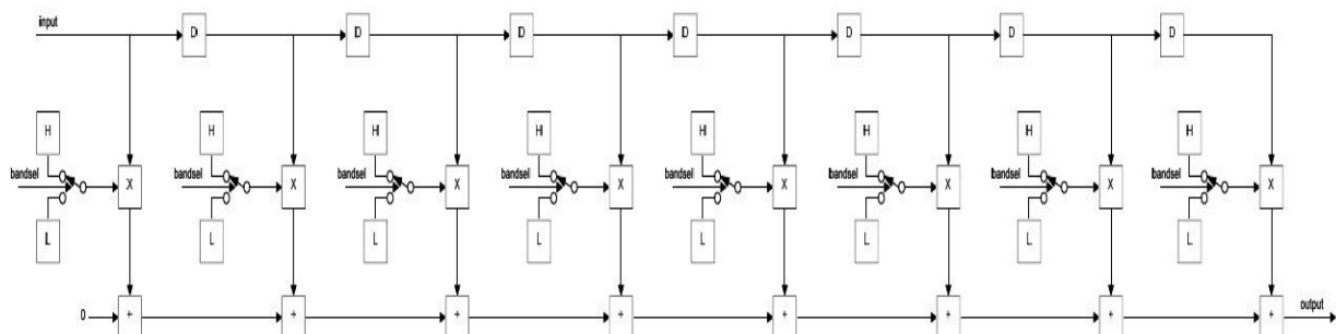
Figure 4: Basic structure of 8 tap FIR filter
