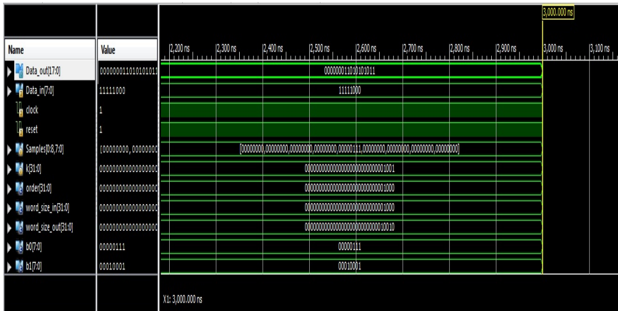
Figure 10: Input and Output waveform of Simulation
