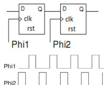
Figure 5: Clock gating of latch-based design
