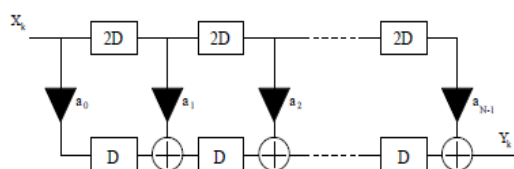
Figure 3: Direct pipe line form of N-tap FIR Filter
