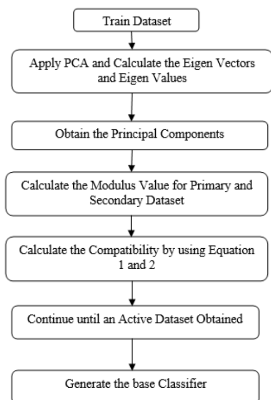
Fig 3. Flowchart for the Proposed Approach.
