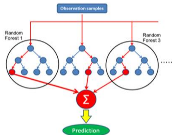
Fig 2. Random Forest Model.
