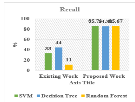
Figure 5 Recall Figure between Existing Work and Proposed Work
