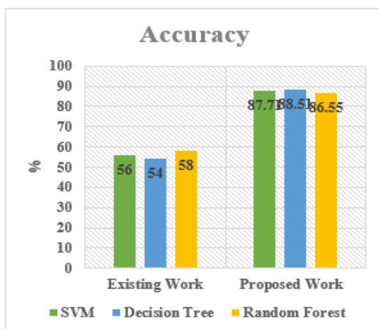
Figure7 Accuracy Figures between Existing Work and Proposed Work.
