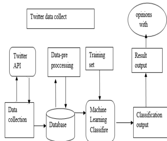
Figure 1. Working Architecture of Twitter classification.
