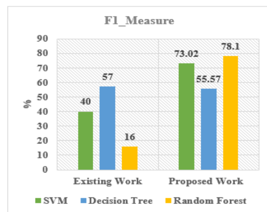
Figure8F1_Score Figures between Existing Work and Proposed Work
