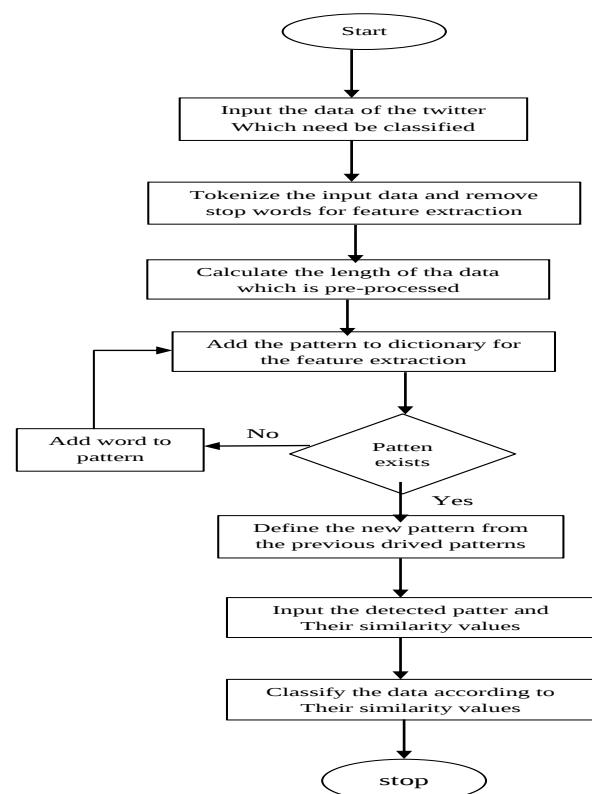
# Training and Testing Figure 2. Proposed Flowchart
