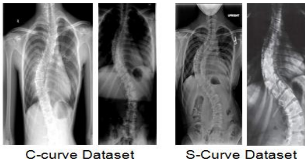
Fig 7. Training Dataset.
