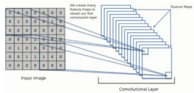
Fig 5. Convolutional Operation
