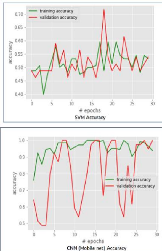
Fig 8. Comparison of accuracies acquired of CNN and SVM algorithms.
