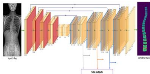
Fig 4. Convolutional Neural Network.
