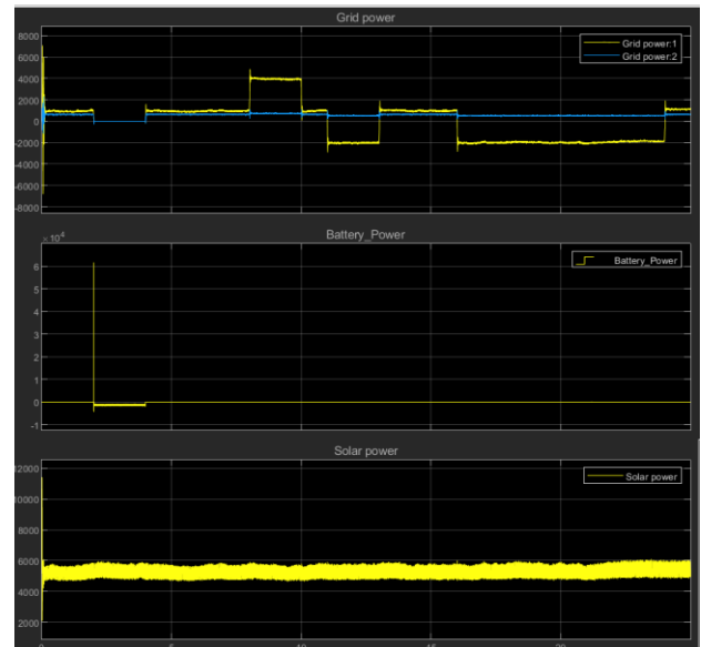
Fig.11 Output usage energy management system.
