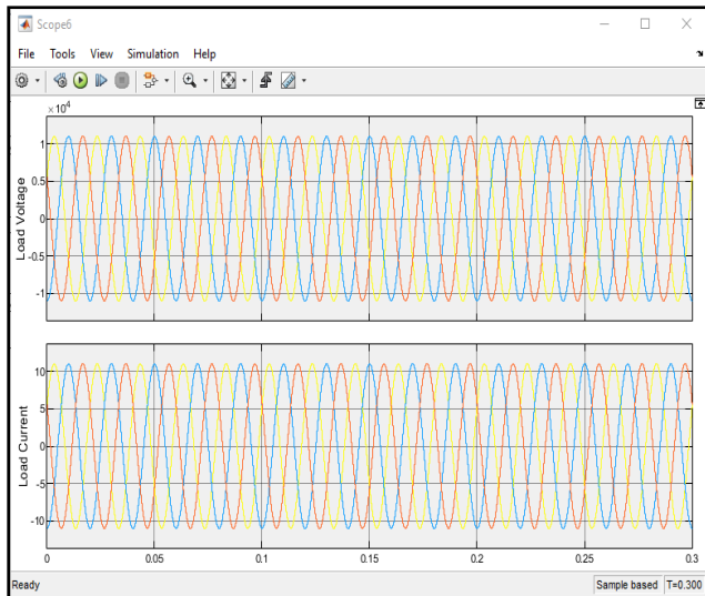
Figure 18: Load Voltage and Current
