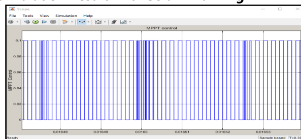
Figure 16: MPPT Control
