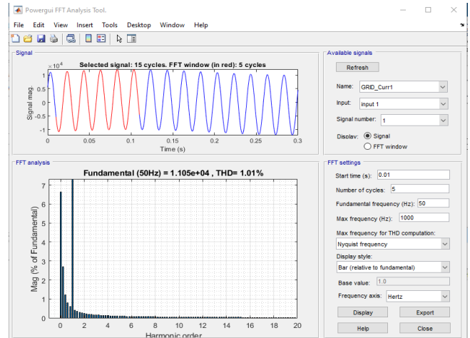
Figure 25 with solar thd
