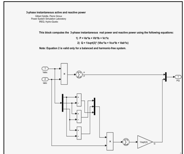
Figure 21: Phase Instantaneous Active and Reactive Power
