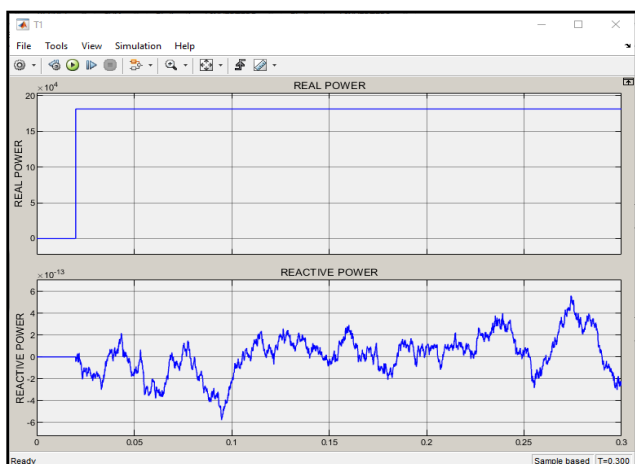
Figure 20: Real Power and Reactive Power
