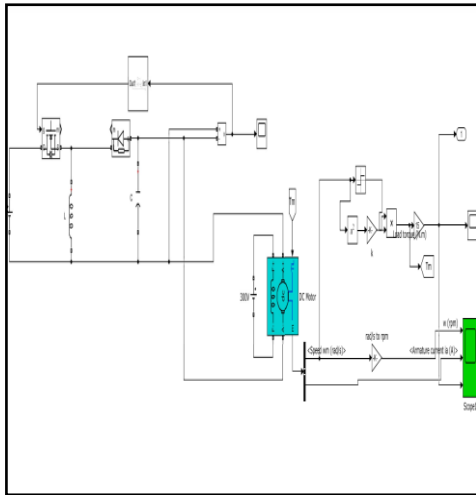
Figure 7: Dc Machine
