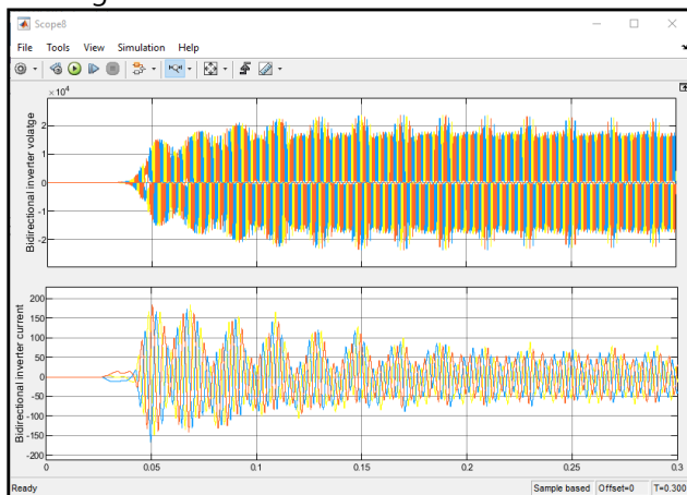
Figure 24: Bidirectional Inverter Current and Voltage
