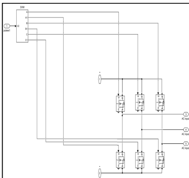
Figure 9: SVM Subsystem
