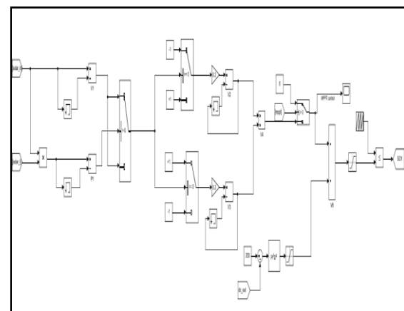
Figure 7: MPPT Control
