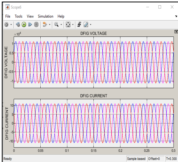
Figure 23: DFIG Voltage and Current
