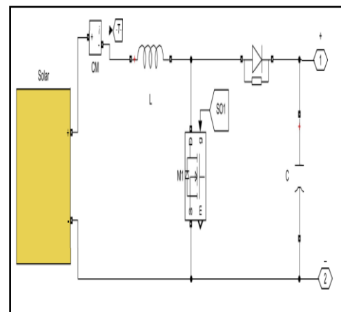
Figure 6: Solar System
