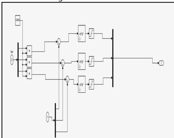
Figure 8: Fractional PID
