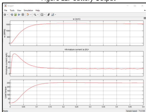
Figure 13: DC Machine Output.
