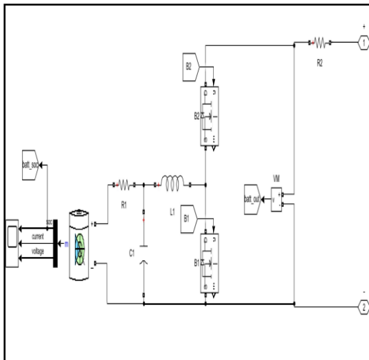
Figure 3: Battery Simulink Model.
