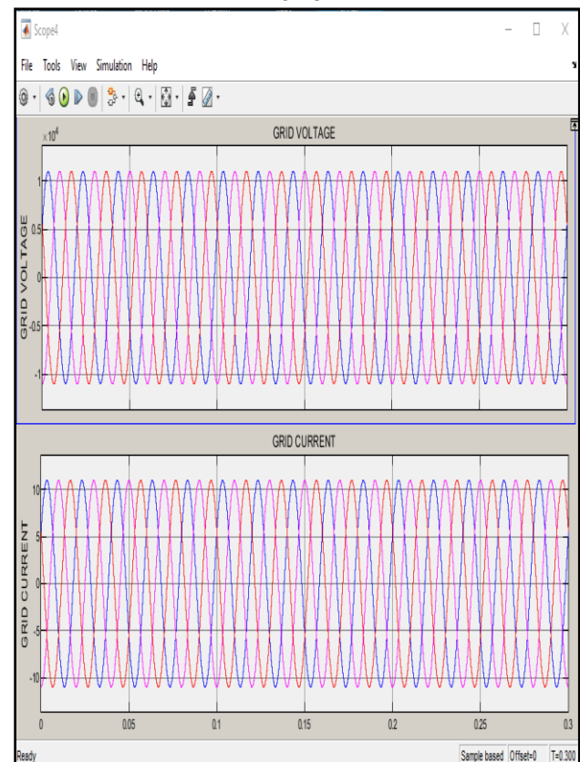
Figure 22: Grid Voltage and Current
