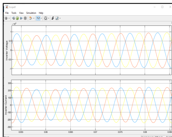
Figure 15: Inverter Current and Voltage.
