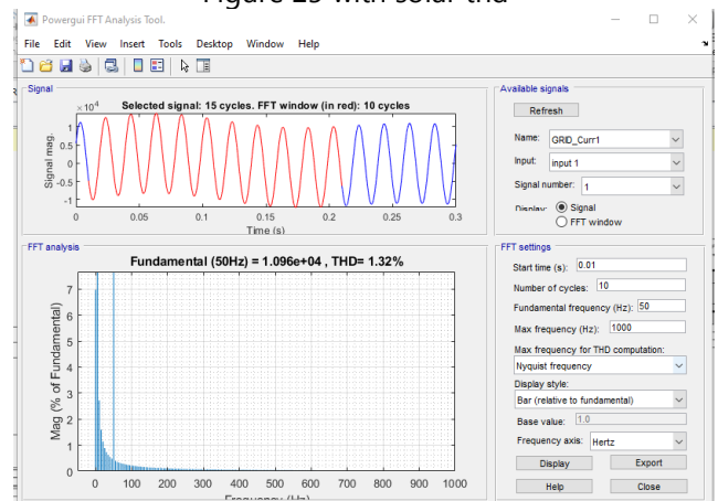
Figure 26 Without solar THD
