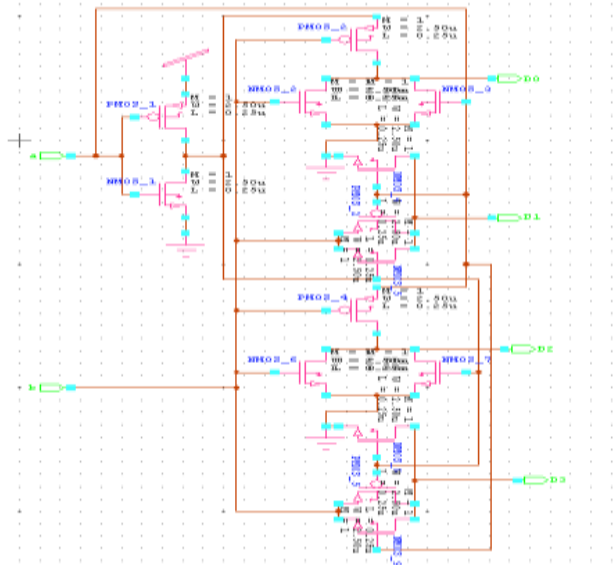
Figure 2: 14T mixed logic Decoder
