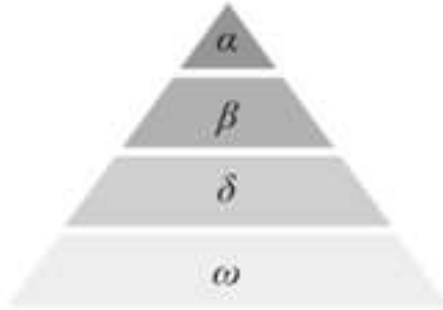
Figure 1: Grey wolf pack ranking
