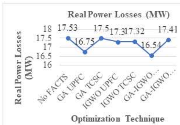
Figure 2: Real power for different optimization techniques
