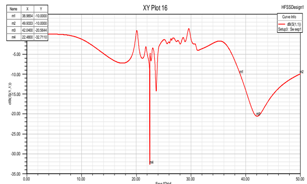
Fig 7 Return Loss of Octagonal Patch Antenna with Ground Slot Antenna.
