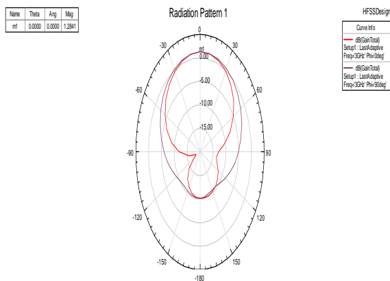
Fig 5 Radiation Pattern of Gain of Octagonal Patch Antenna.
