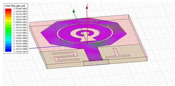
Fig 8 Current Distribution of Octagonal Patch Antenna with Ground Slot Antenna on Patch.
