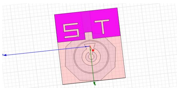
Fig 6 Top View of Octagonal Patch Antenna with Ground Slot.
