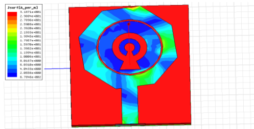
Fig 4 Current Distribution of Octagonal Patch Antenna.
