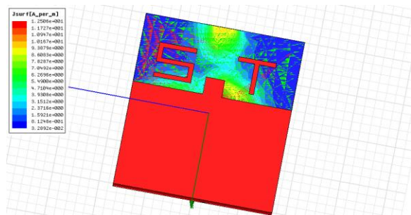
Fig 9 Current Distribution of Octagonal Patch Antenna with Ground Slot Antenna on ground.
