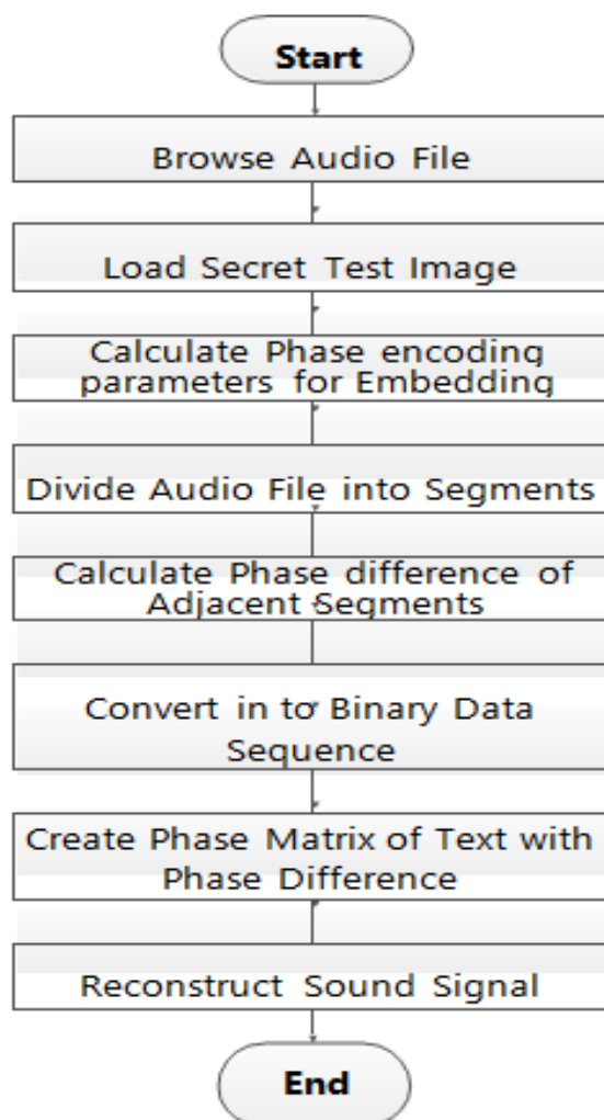
Fig 3. Flow Chart of Embedding Process.
