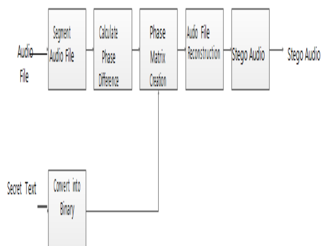
Fig 2. Block Diagram of Embedding Process.
