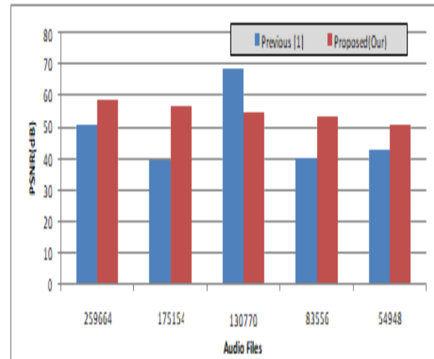
Fig 6. PSNR Comparison Chart.
