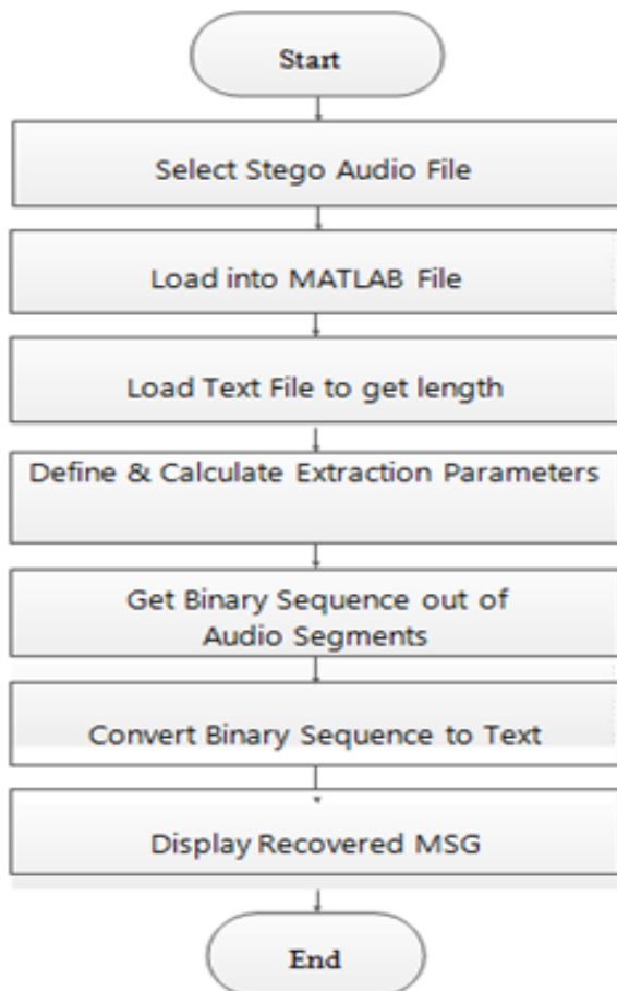
Fig 5. Flow Chart of Extraction Process.
