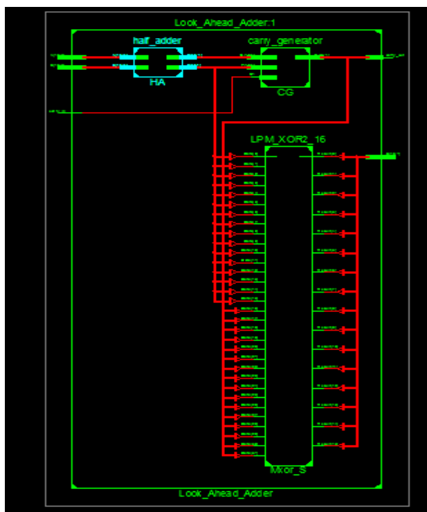
Figure.7 RTL view of 16-bit carry look ahead adder
