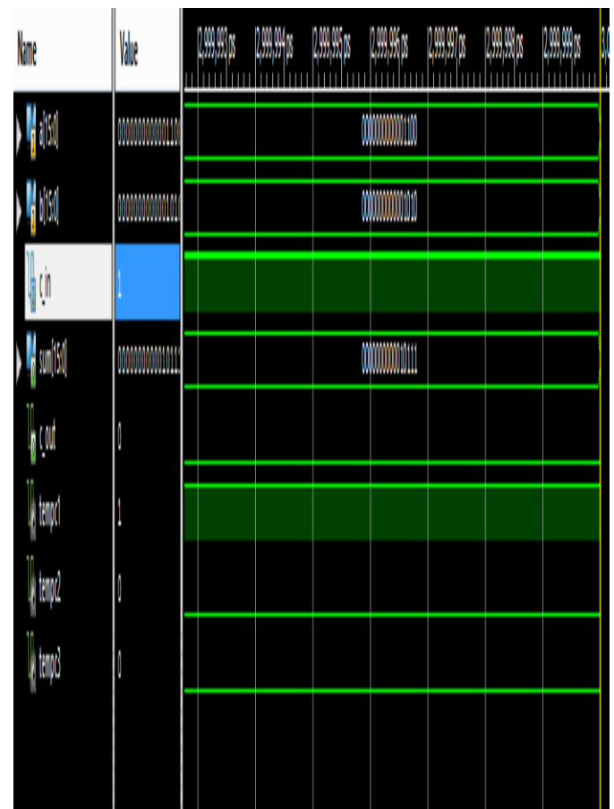
Figure.10 Simulation result of adder design
