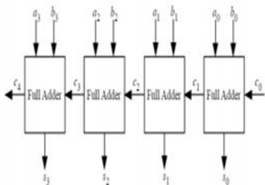
Figure 1 Full adder
