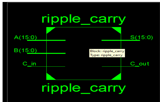
Figure.4 RTL view of 16-bit ripple carry adder.
