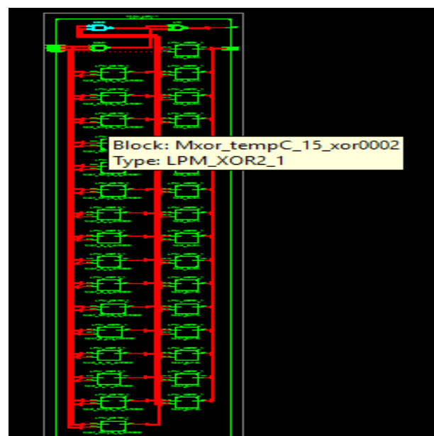
Figure.5 RTL view of 16-bit ripple carry adder
