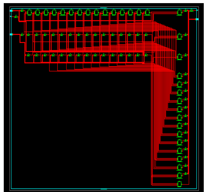
Figure.8 Technological schematic of adder design
