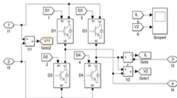
Fig 3. Simulation model of Inverter Unit.
