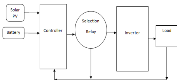
Fig 1. Functional Block Diagram of Standalone system.
