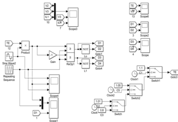
Fig 4. PWM Pulse Scheme for inverter and controller operation.
