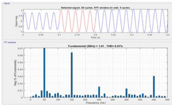
Fig 10. Load Current FFT.
