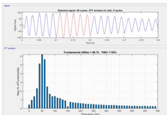
Fig 11. Load Voltage FFT.
