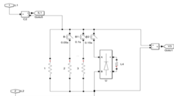
Fig 5. Load variation Unit with controller operation.
