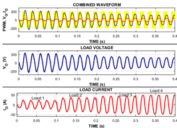
Fig 7. Output voltage and current waveforms without control action.
