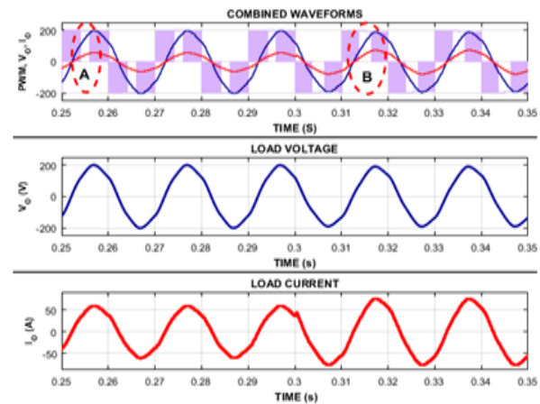
Fig 9. Observed change in Pulse Width with change in load.
