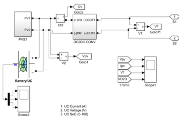
Fig 2. Simulation model of PV- Battery/UC system with DC-DC converter Unit.
