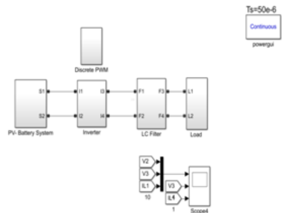
Fig 6. Simulation model of proposed PV system.
