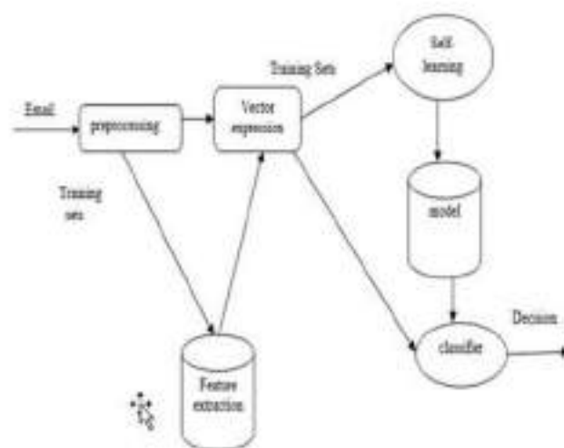
Fig 2. Spam Filtering Architecture by Applying Machine Learning Techniques.
