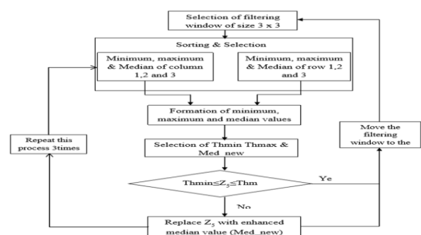
Fig. 6: Block Diagram of Threshold Filter
