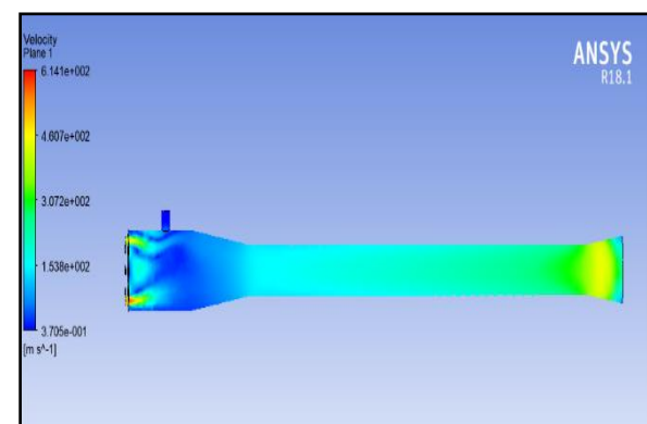
Fig 7. Velocity plot of single fuel inlet design.
