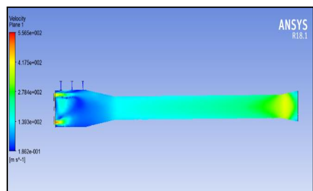
Fig 13. Velocity plot with three fuel inlet in vertical configuration.
