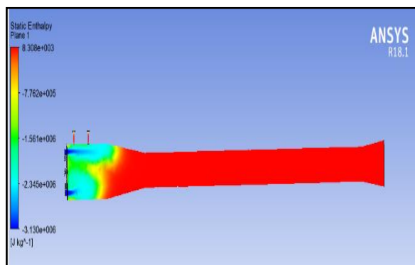
Fig 11. Static enthalpy plot with double fuel inlet in vertical configuration.
