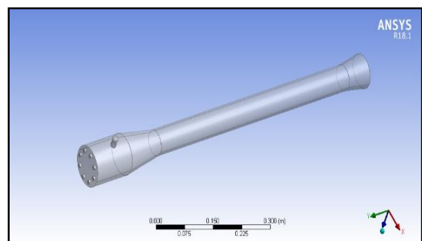
Fig 2. CAD Model of Pulsejet Engine.
