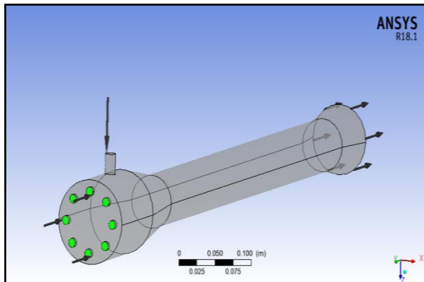
Fig 4. Air Inlet Definition.
