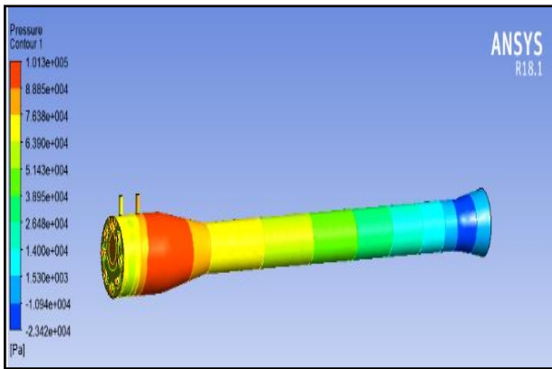
Fig 9. Pressure plot with double fuel inlet in vertical configuration.
