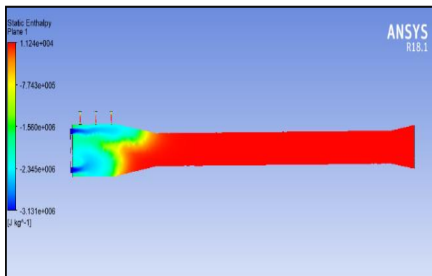
Fig 14. Static enthalpy plot with three fuel inlet in vertical configuration.
