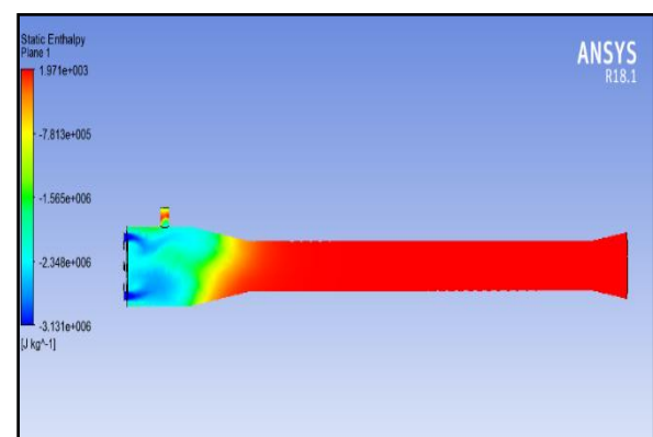
Fig 8. Static Enthalpy using single fuel inlet.
