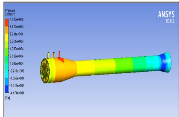
Fig 12. Pressure plot with three fuel inlet in vertical configuration.
