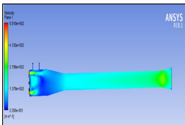
Fig 10. Velocity plot with double fuel inlet in vertical configuration.
