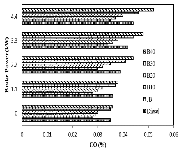
Fig 3. CO Variation With Load.
