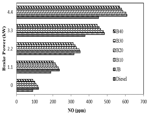
Fig 4. NO Emission Variations With Load.
