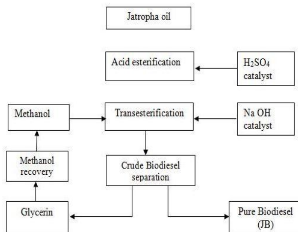
Fig 1. Transesterification Process.
