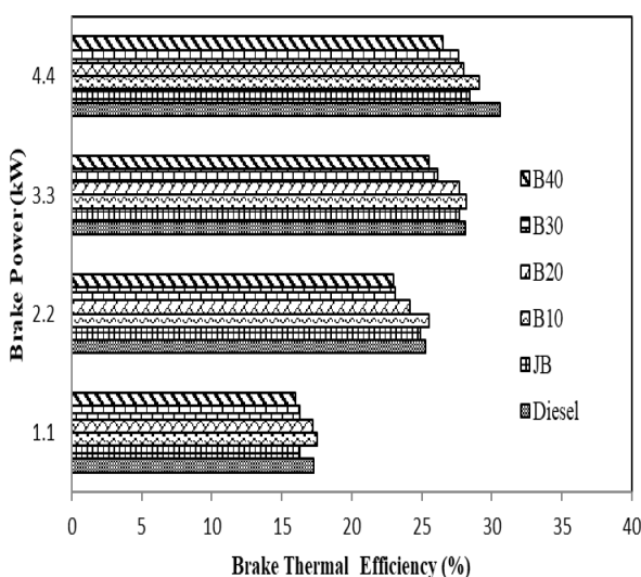
Fig 5. BTE Variation Along With Load.
