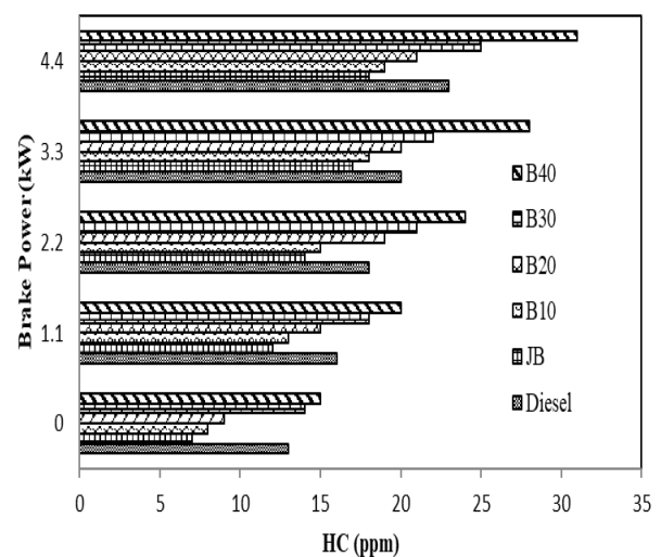
Fig 2. HC Variations.
