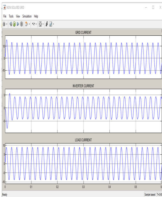
Fig. 19 inverter current, grid current, load current
