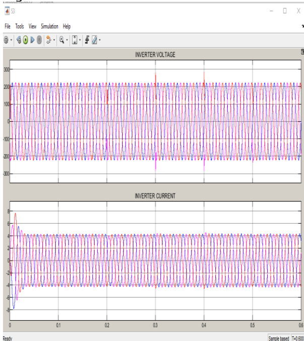
Fig. 16 inverter current and voltage
