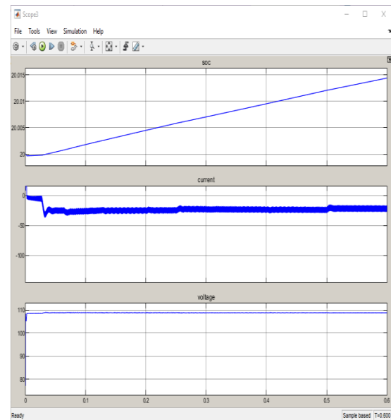
Fig. 21 battery current and voltage
