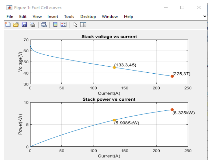
Fig 22 fuel cell voltage and current.
