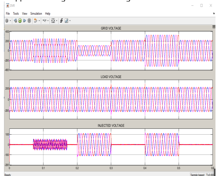
Fig 18 Grid disturbance as swell, sag, , harmonics, and load voltage and injected voltage :
