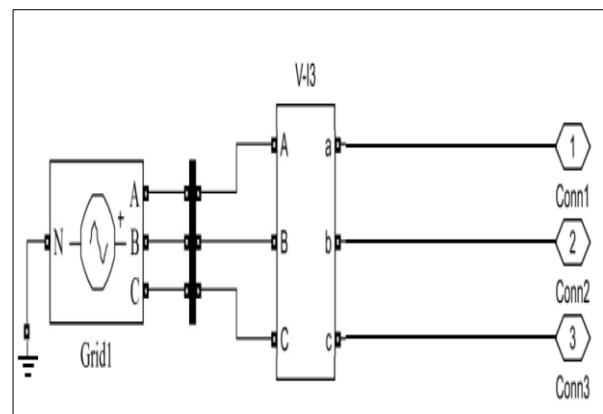
Fig 11 Grid subsystem
