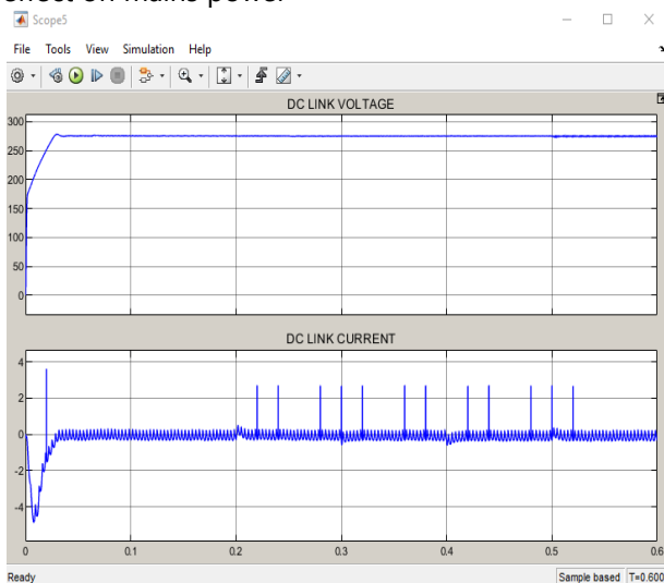
Fig 20 DC link output.
