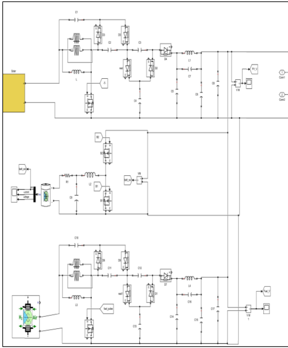
Fig.3 solar, battery and fuel. Table 1 Solar Parameters
