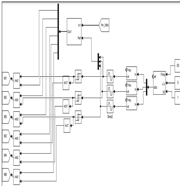
Fig 12 grid inverter synchronization subsystem
