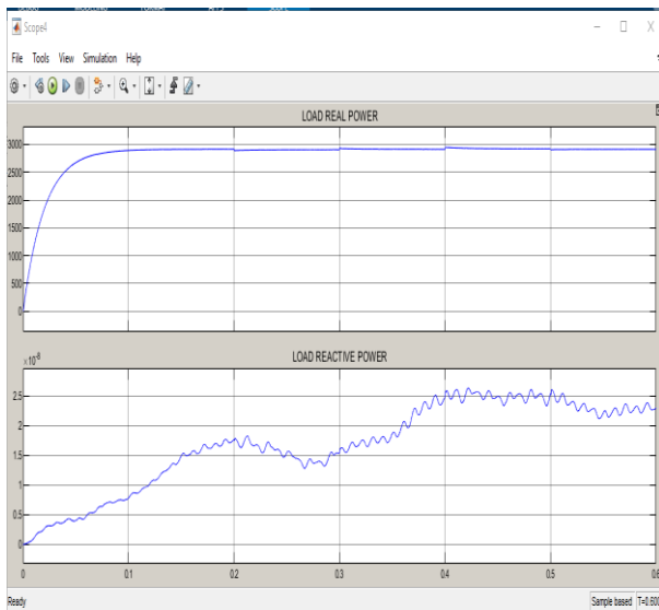
Fig.15 load real power and reactive power
