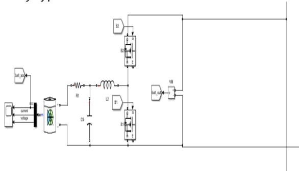
Fig .7 battery model
