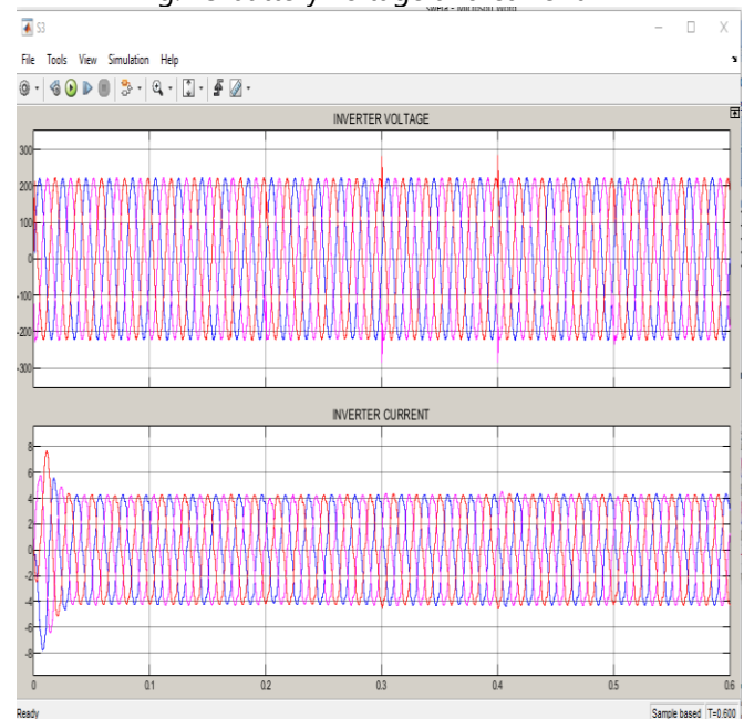
Fig.14 inverter current and voltage.
