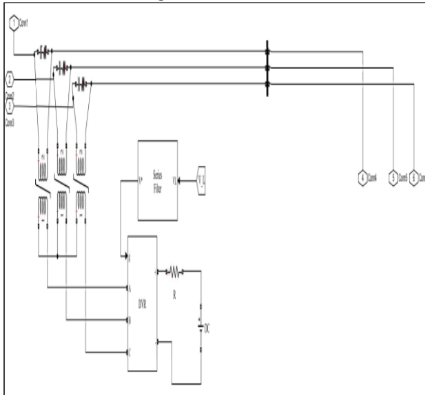
Fig.10 DVR Subsystem
