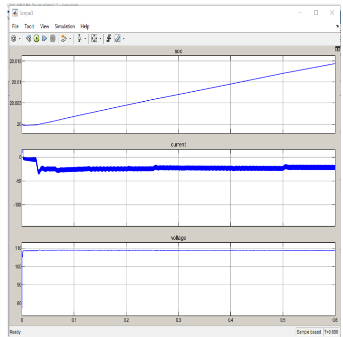
Fig. 13 battery voltage and current
