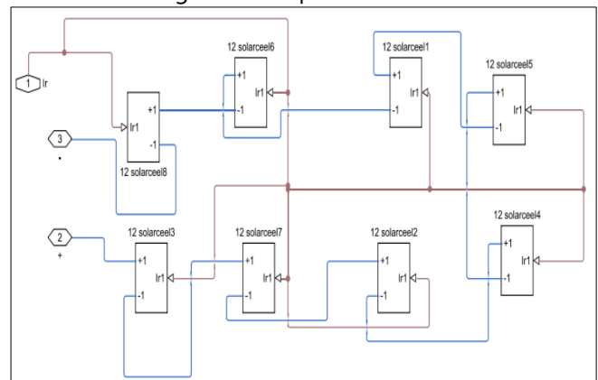
Fig. 6 solar cell subsystem
