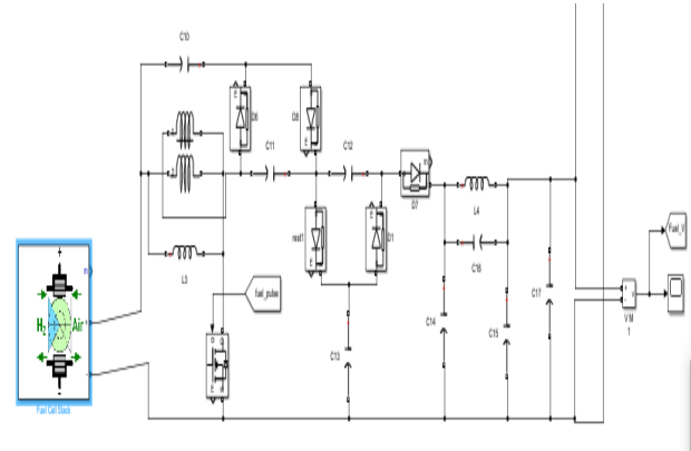
Fig 8fuel cell subsystem
