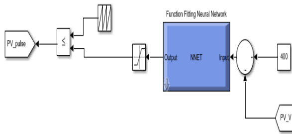
Fig 9 ANN Controller
